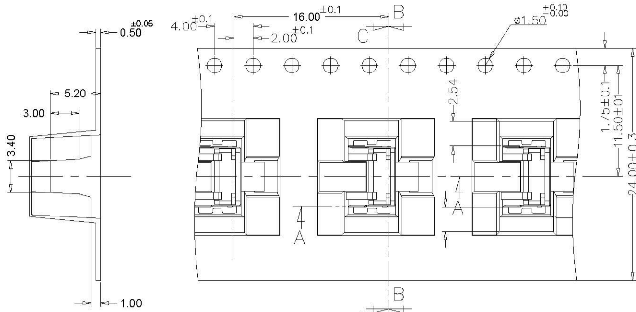
C-C Section
