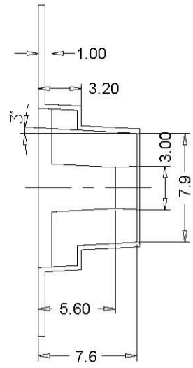
B-B Section
